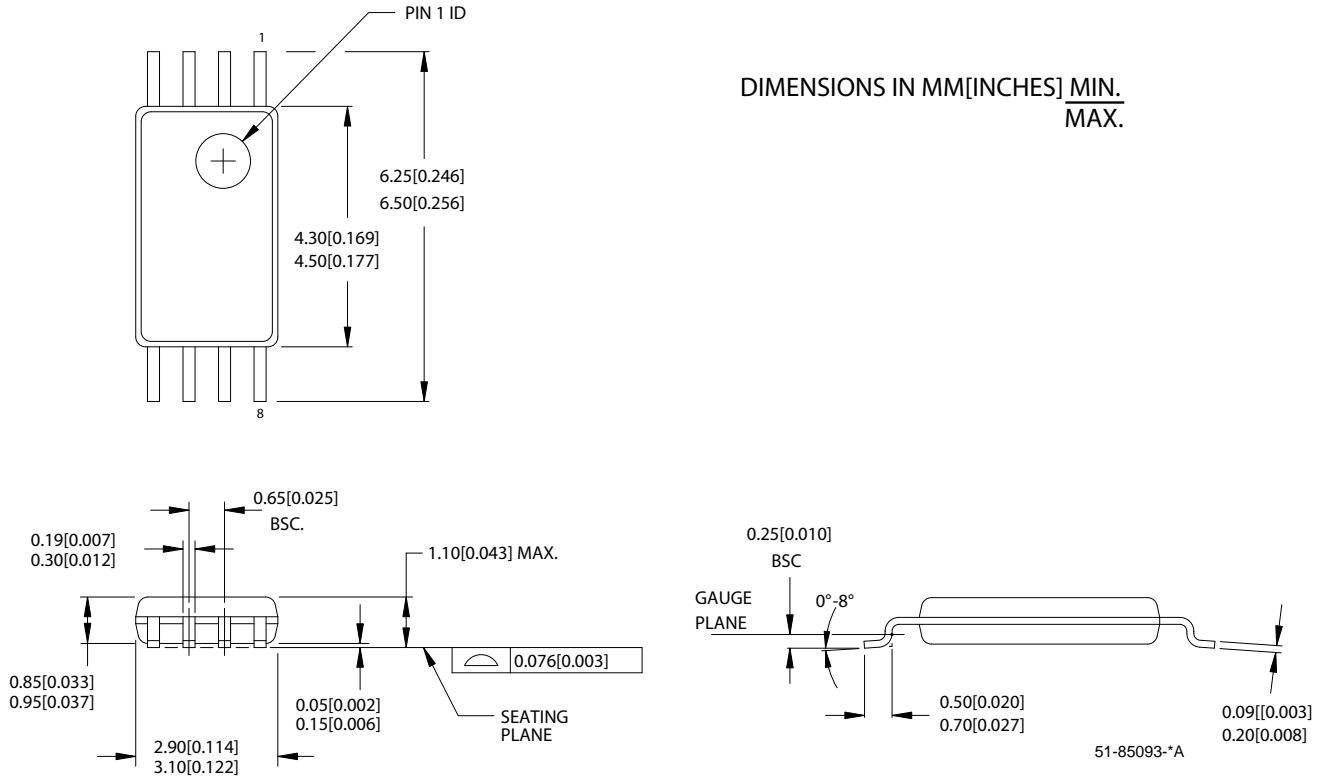
Figure 6. 8-Pin Thin Shrunk Small Outline Package (4.40 MM Body) Z8 (51-85093)
